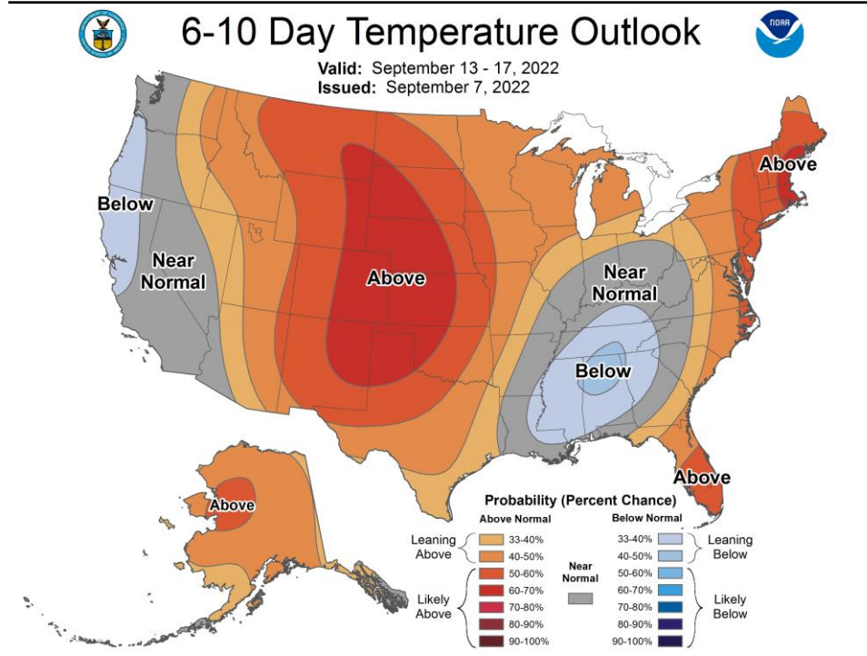
图7、0913-0917气温前瞻
